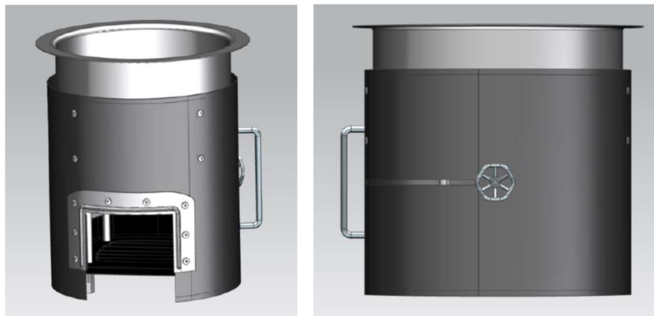
Baldwin stove
